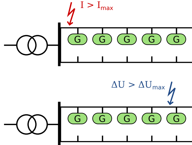
Figure 4: Locations of electricity networks at which thermal limits (top) and and voltage limits (bottom) are typically violated. The letter G denotes generation units such as renewable energy power plants. Figure adapted from dena (2012).
