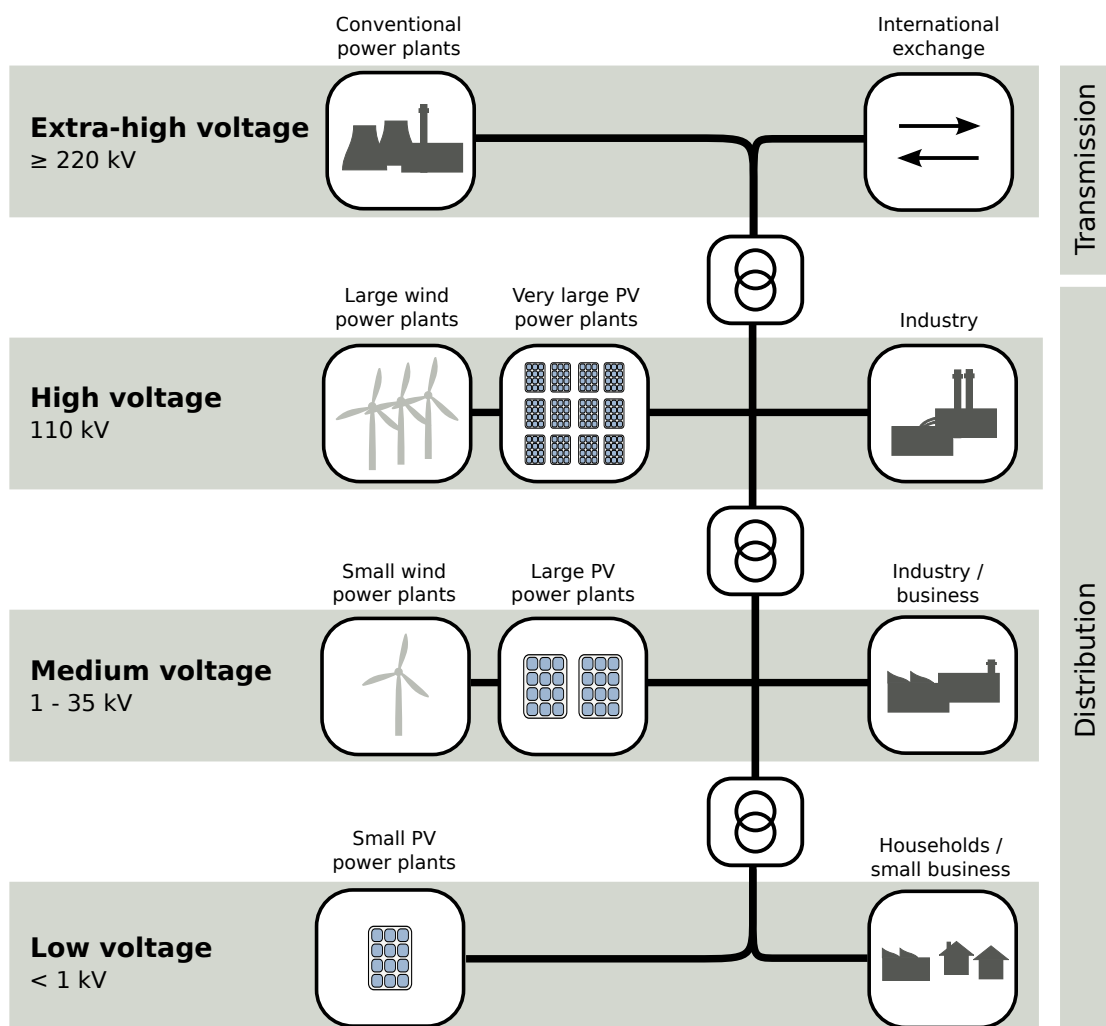
Figure 1: The German power system can be divided into the transmission and the distribution system, each with different voltage levels. For simplification, only two technologies for generating electricity from renewable resources are shown. Figure adapted from Gust (2014).
