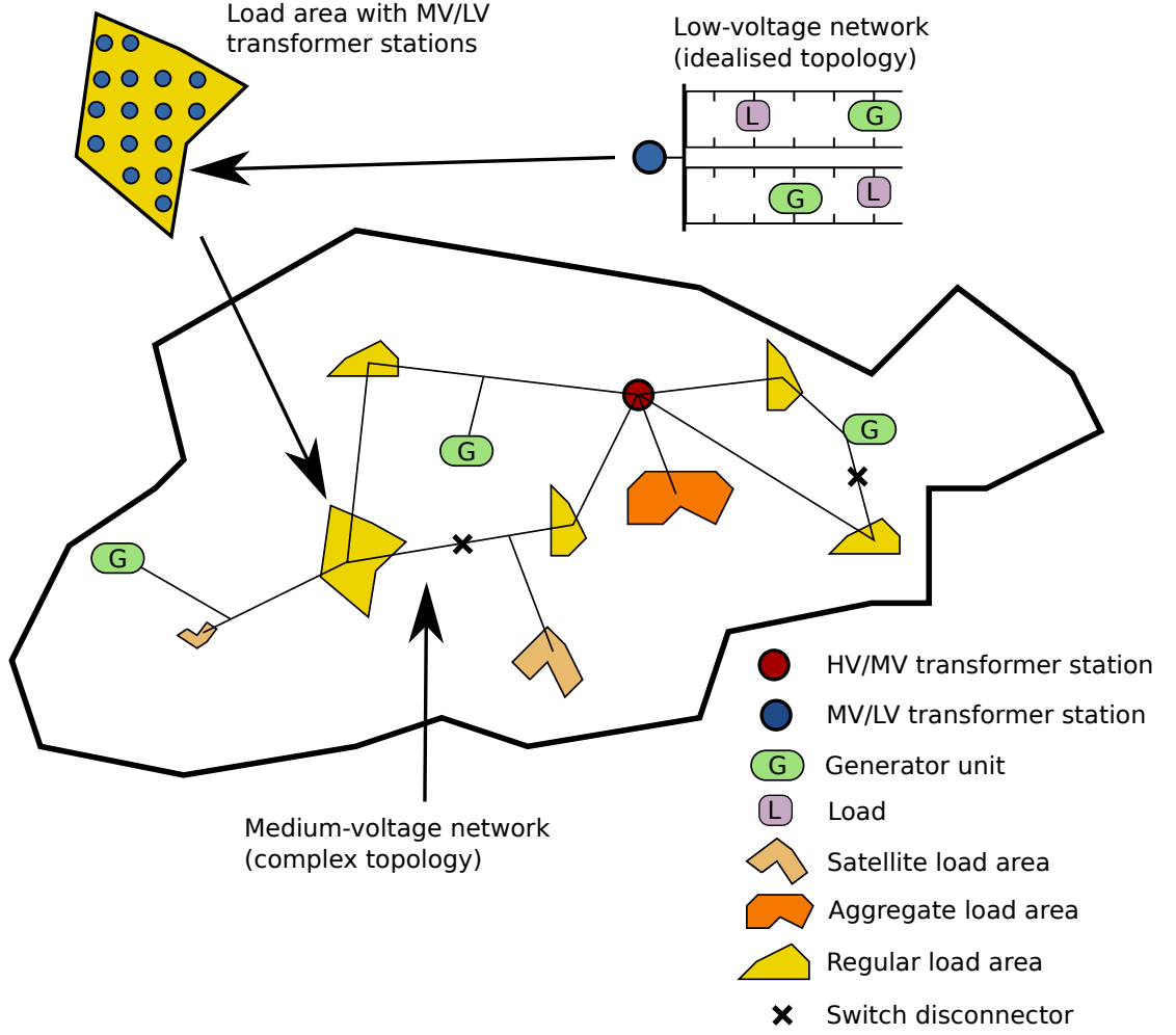
Figure 8: Schematic illustration of medium-voltage network district with load areas, low-voltage network districts and low-voltage networks. Figure based on Amme et al. (2017).
