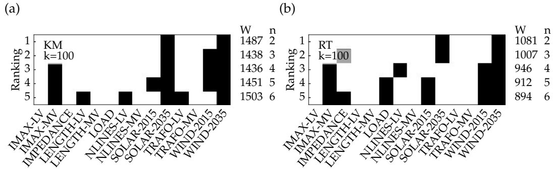
Figure 19: The best cluster model with K = 100 and n = 2, 3, \dots, 6 according to W for (a) K-Mean and (b) regression tree estimation.
