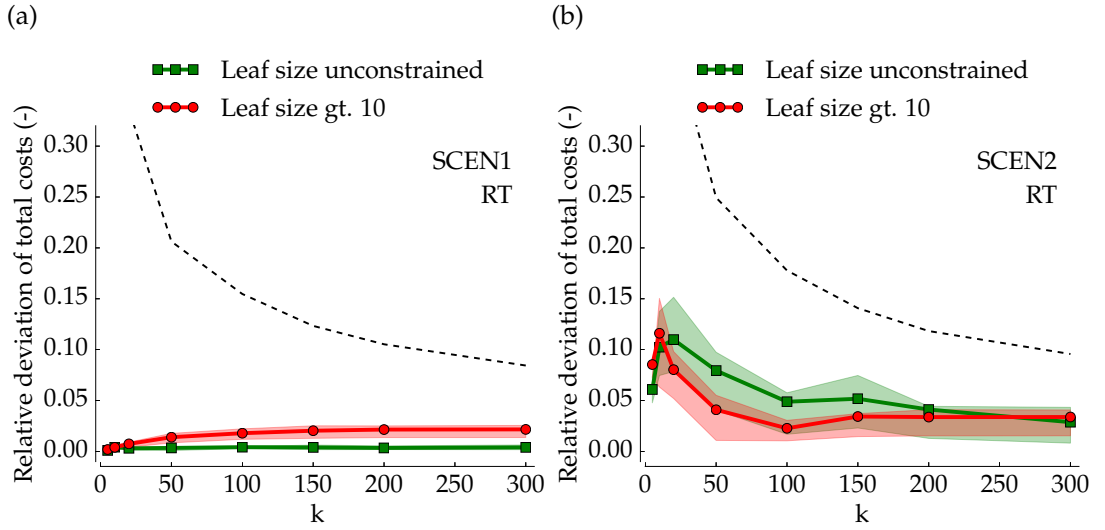
Figure 31: Relative deviation of estimated total costs from total costs ( R in Equation 5.12) for different number of clusters K and for the (a) worst-case scenario and (b) curtailment scenario. Lines indicate arithmetic mean for a subset of the 28 cluster models in Section 6.4, shaded area ranges from 25 percentile to 75 percentile of these models. The black dashed line indicates the mean relative deviation for random samples of size K (see Figure 20). Regression tree estimation (RT) with size of leafs unconstrained (green color) and size of leafs n_k > 10 (red color).
