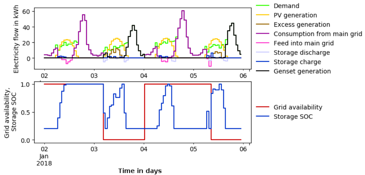
Figure 4.6.: Energy flows in off-grid MG connected to unreliable central grid ( nosp 3670 )
